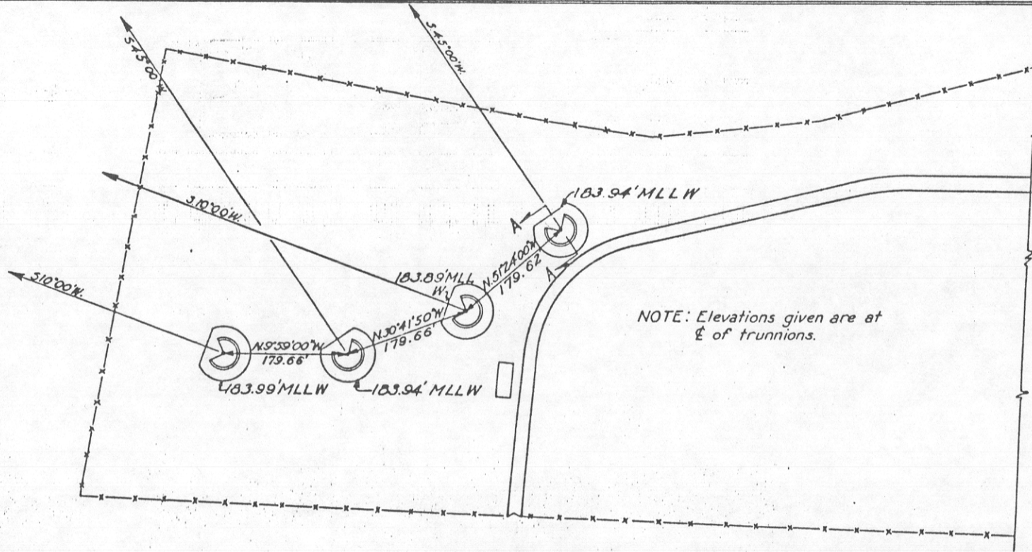
LOCATION PLAN
