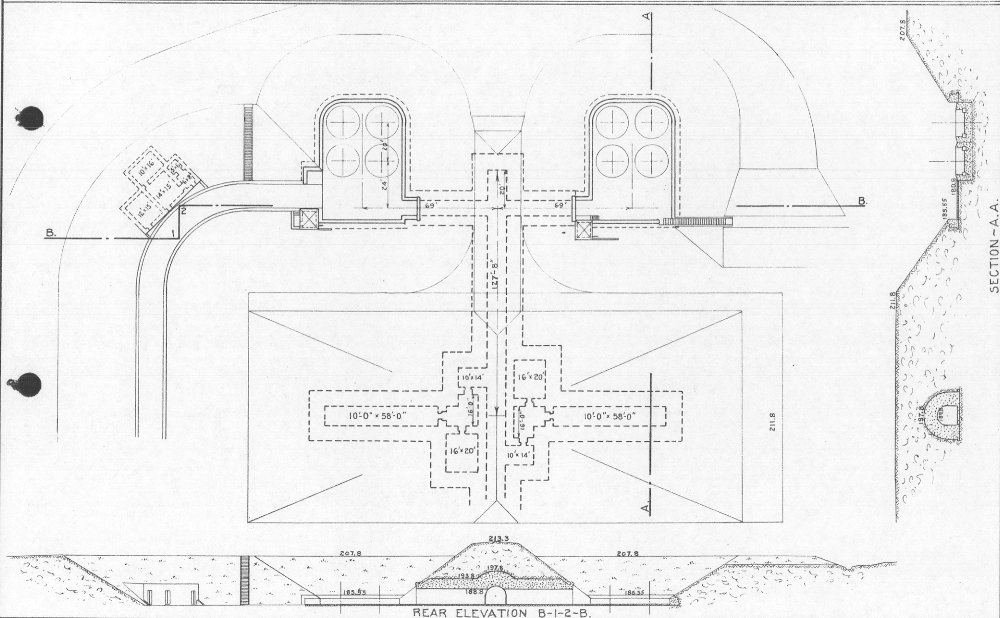
REAR ELEVATION B-1-2-B.
