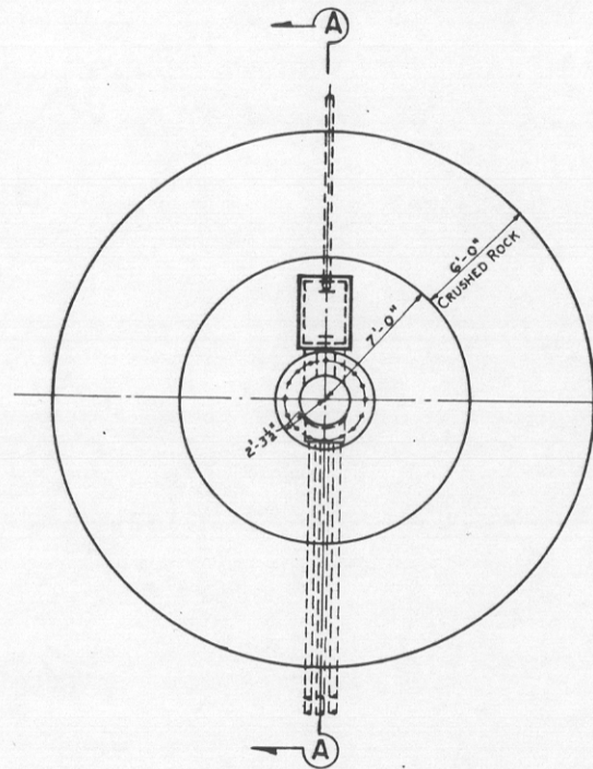
PLAN OF GUN BLOCK
